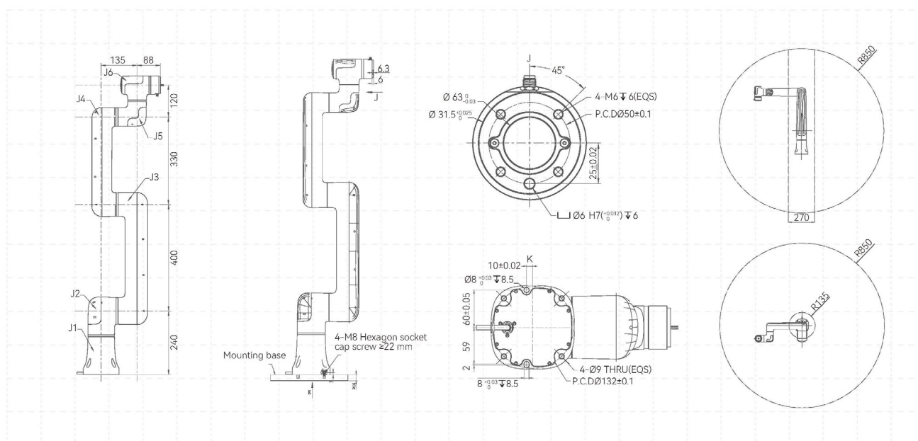
Overall dimension diagram
